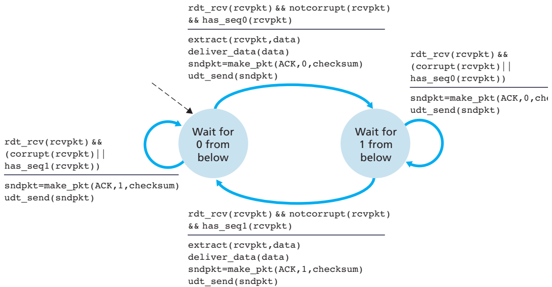
Figure 3.14 ♦ rdt2.2 receiver
